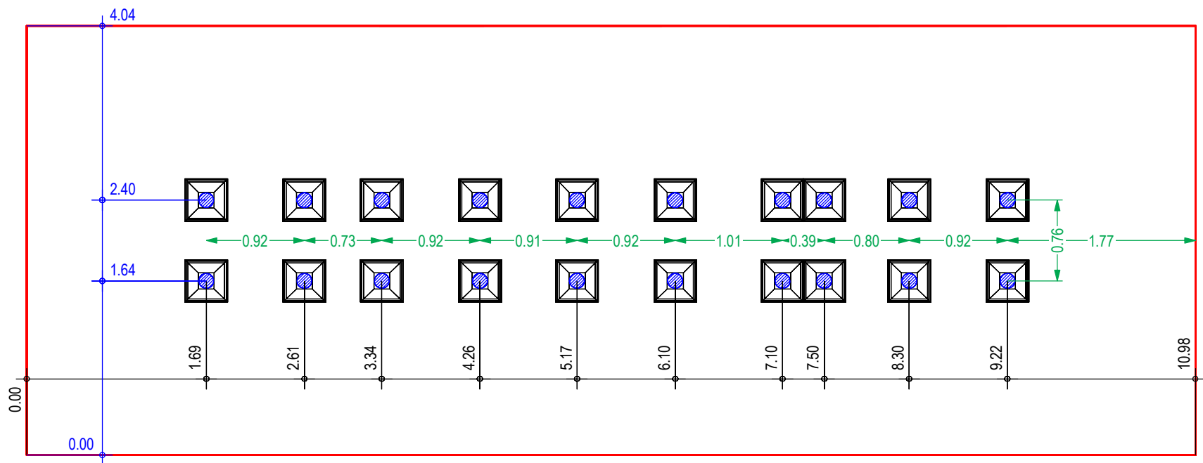
Alternativ: Fundament flach/kantig (Alternative: Foundations plain/edged)
