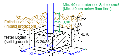
Alternativ: Fundament flach/kantig (Alternative: Foundations plain/edged)
